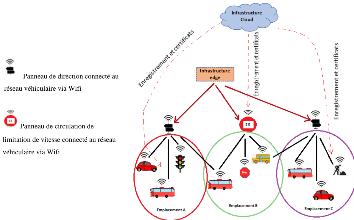
Figure 2 : Architecture Cloudlets de confiance de communication V2V
